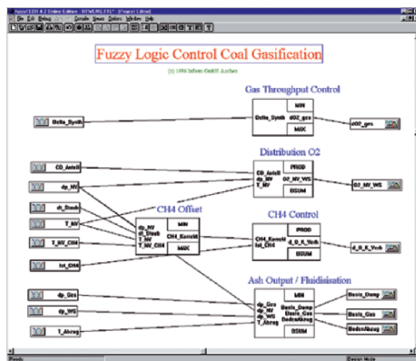
Fig. 8.3. Fuzzy controller structure
