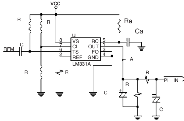
Fig. 9.46. The circuit of F/V converter
