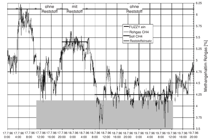
Fig. 8.8. Process stabilization
