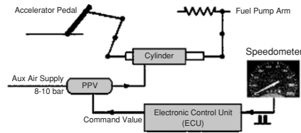
Fig. 8.35. Mechanical design of the speed limiter
