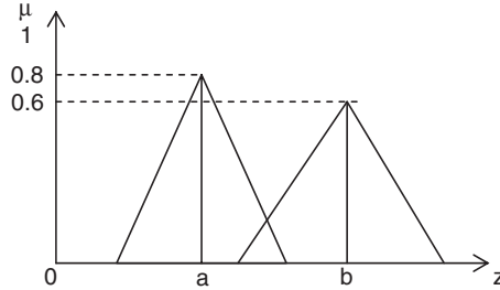
Fig. 5.4. Weighted average method
