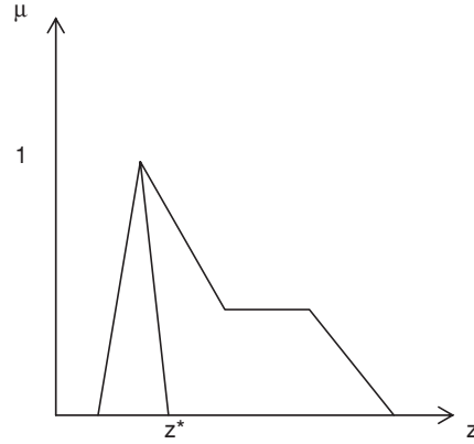
Fig. 5.2. Max-membership method
